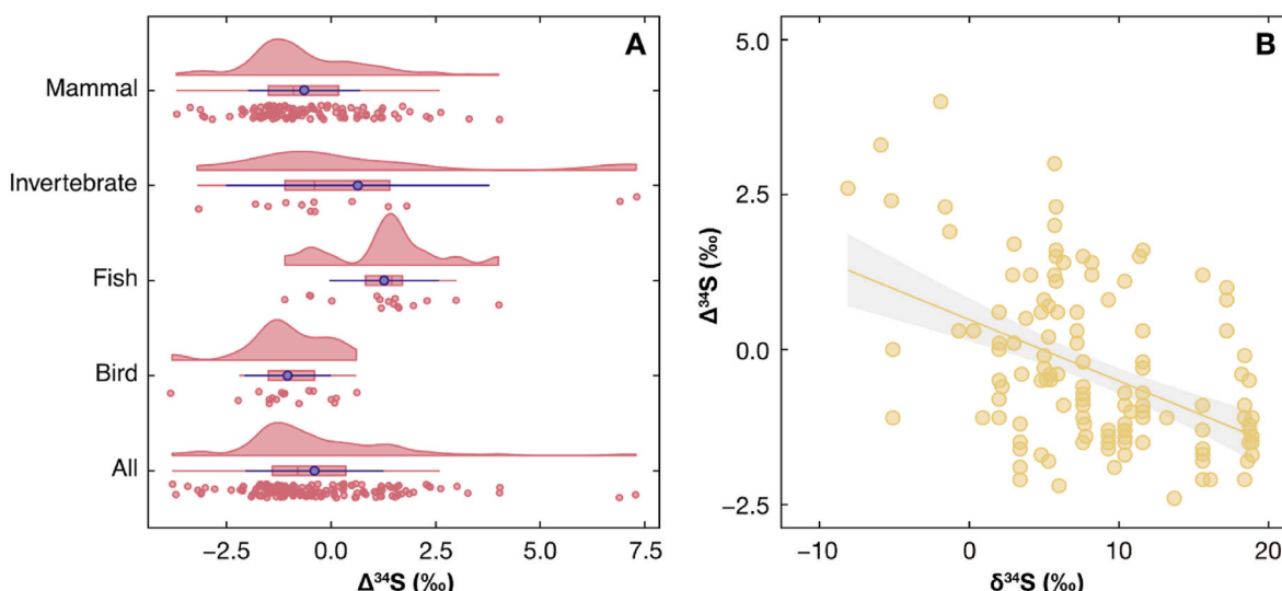
Fig. 3. A) Variation in estimates of \Delta^{34}\text{S} , the tissue-diet trophic discrimination factor (TDF) for sulfur estimated for different taxa including birds, fish, invertebrates, and mammals, and for all tax combined. Each marker relates to an individual empirical estimate from the literature for a certain feeding experiment of condition. Red circles and lines mark the estimated mean \pm SD \Delta^{34}\text{S} for a given taxon (values given in the main text), while the boxplots show the median \pm IQR. A vertical line marks the commonly used zero value of \Delta^{34}\text{S} . B) Shows a noisy ( R^2 = 0.2 ) but significant negative relationship between mean \Delta^{34}\text{S} and the mean \delta^{34}\text{S} value of experimental diet fed to consumers in each experiment. The regression equation is \Delta^{34}\text{S} = 0.43 (\pm 0.19) - 0.11 (\pm 0.02) \times \delta^{34}\text{S}_{\text{diet}} , F_{1,140} = 36.3 , R^2 = 0.20 , P < 0.0001 . (For interpretation of the references to color in this figure legend, the reader is referred to the Web version of this article.)
